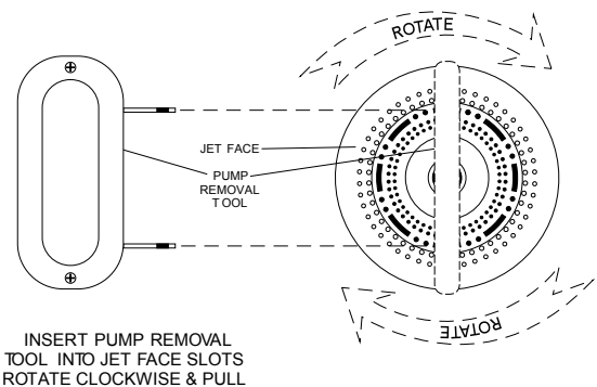
PUMP REMOVAL
