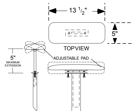
FOOTREST
