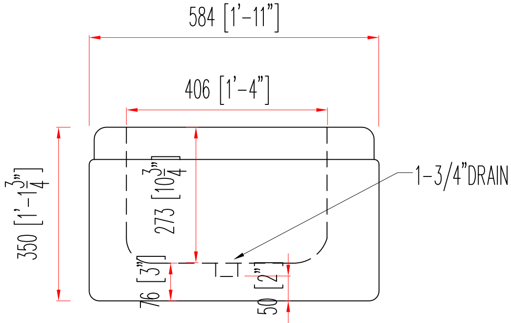
SIDE VIEW
