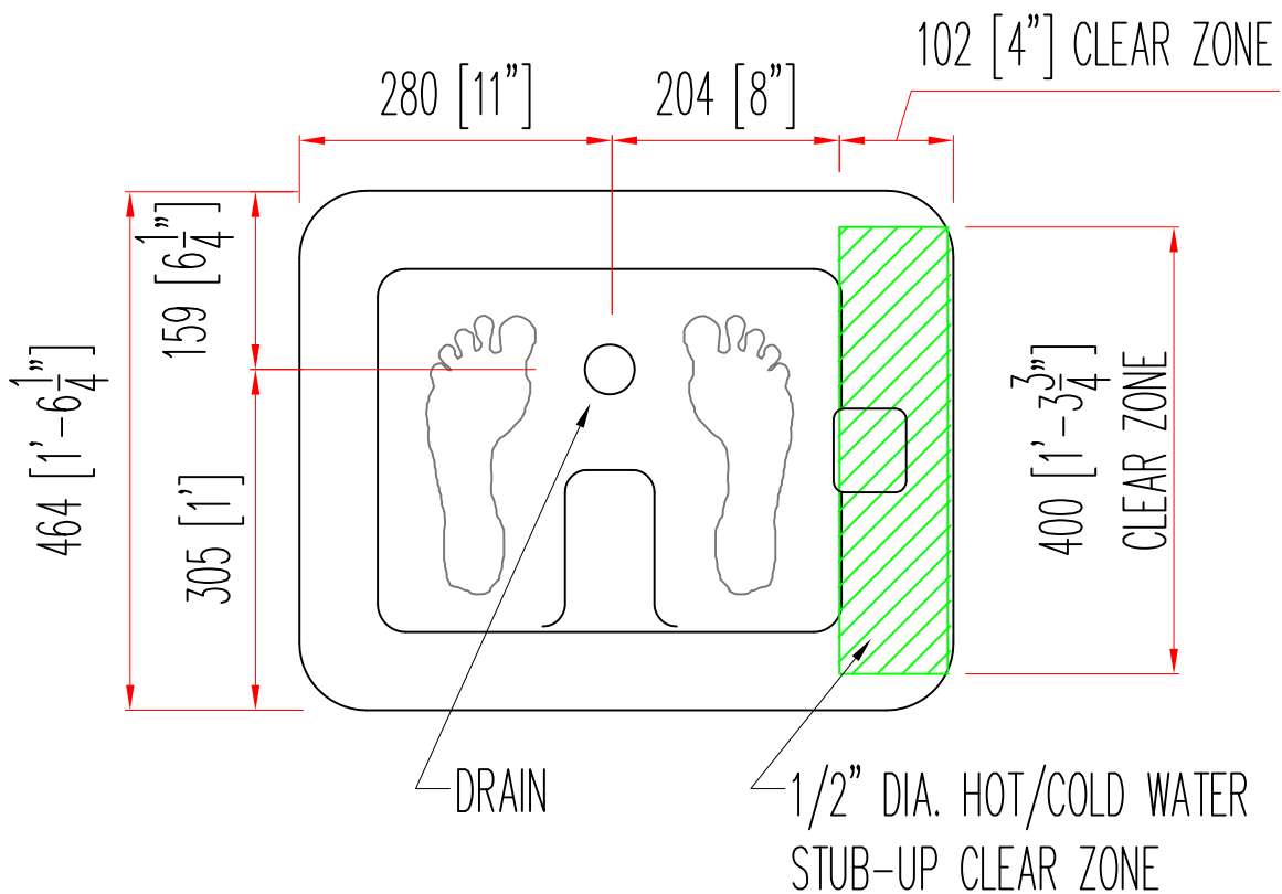
TOP VIEW
