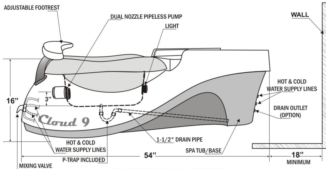
ALL DIMENSIONS ARE APPROXIMATE SIDE VIEW
