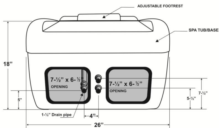
ALL DIMENSIONS ARE APPROXIMATE BACK VIEW
