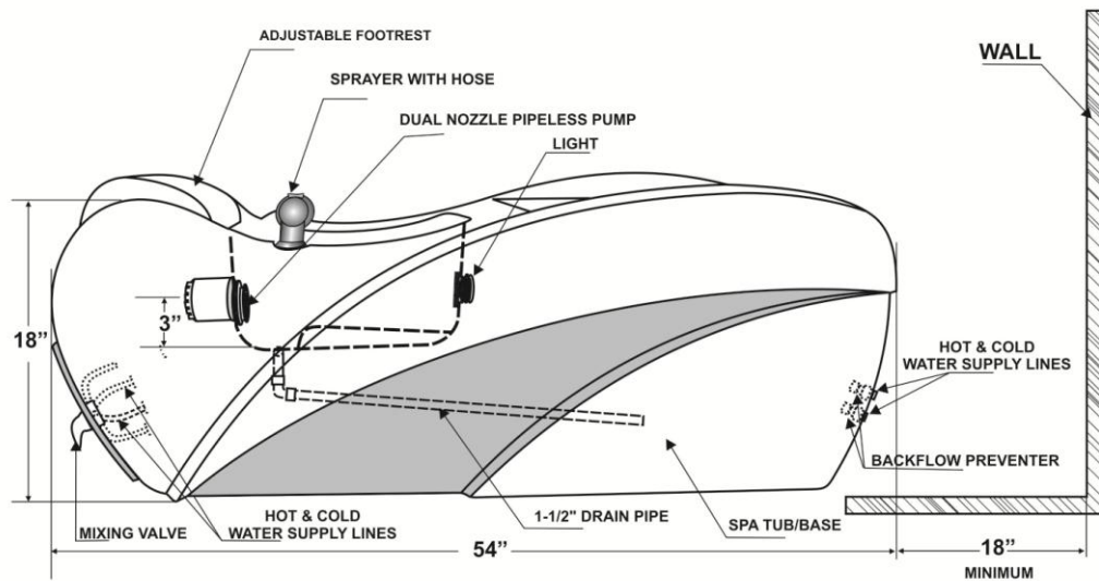
ALL DIMENSIONS ARE APPROXIMATE SIDE VIEW
