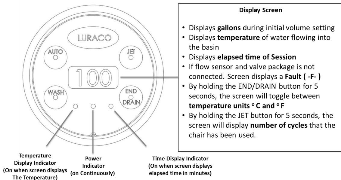
Fig.2: Display Screen
