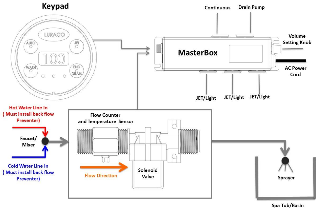
Fig.1: Connection Diagram
