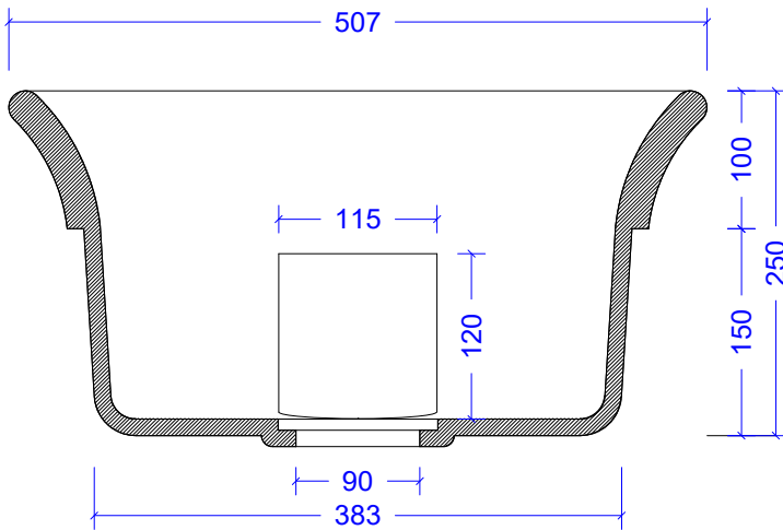
02 PEDIPOT® SECTION VIEW 2" = 1'
