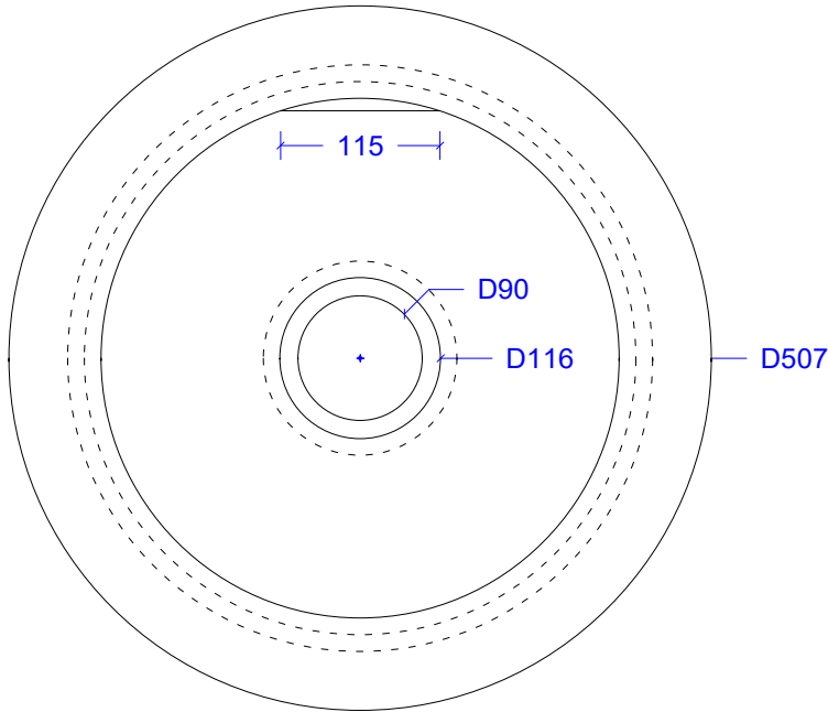
01 PEDIPOT® PLAN VIEW 2" = 1'
