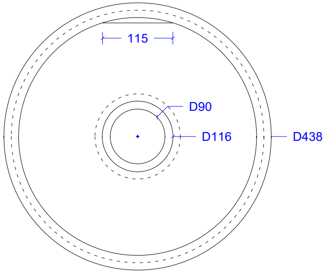
01 PEDITUBE® PLAN VIEW 2" = 1'
