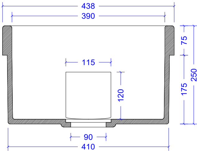
02 PEDITUBE® SECTION VIEW 2" = 1'
